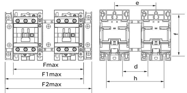
图8RDC5-40N~95N
