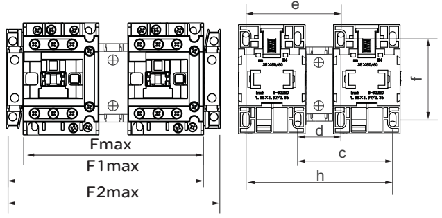
图7RDC5-06N~38N
