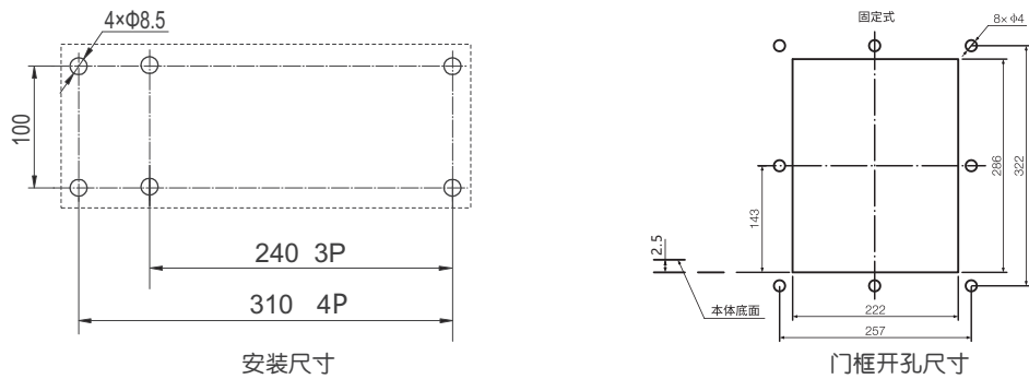
RDW5-1000S/H~1600S安装尺寸
