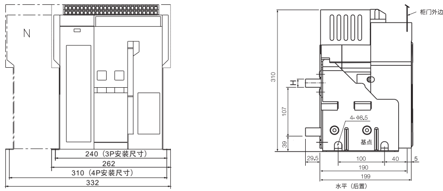
RDW5-1000S/H~1600S安装尺寸
