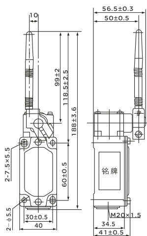
图9 L XK3-20S/D
