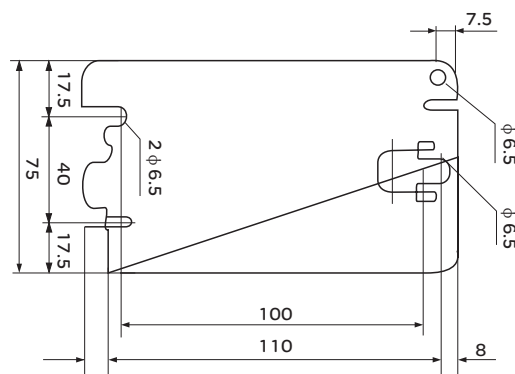
CJX2s-40, 50, 65, 80, 95
